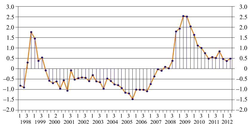
Chart 5 Latvian FSI (Q1 1998–Q3 2012; in standard deviations)
